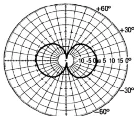
Diagrama de Radiación Vertical Vertical Radiation Pattern
